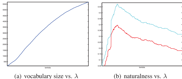
Figure 2. Left: shows the relationship between parameter \lambda and the target vocabulary size. Right: shows the relationship between parameter \lambda and agreement accuracy with human labeled synsets evaluated against the most agreed human label (red) and any human label (cyan).
